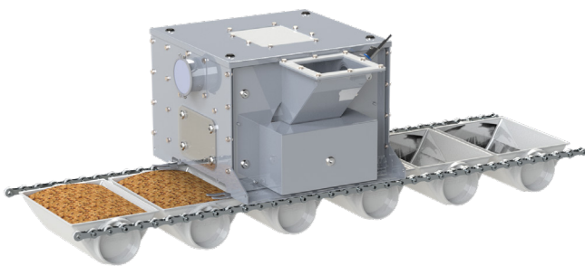
Drum feeder
