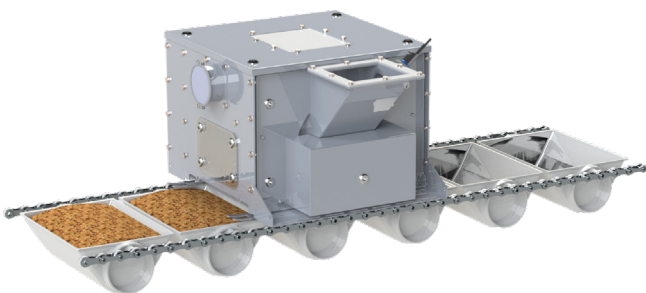
Drum feeder
