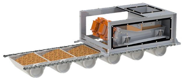
Vibrating feeder
